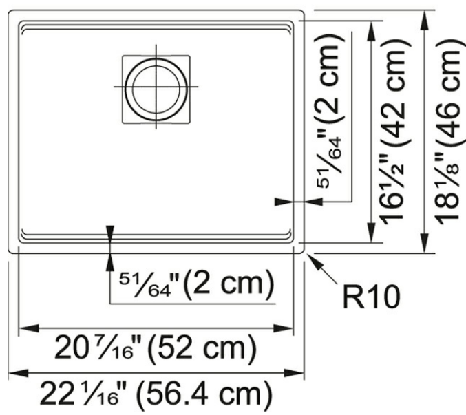
Technical Drawing
