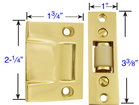
Roller Catch with Strike & Screws (8801)
