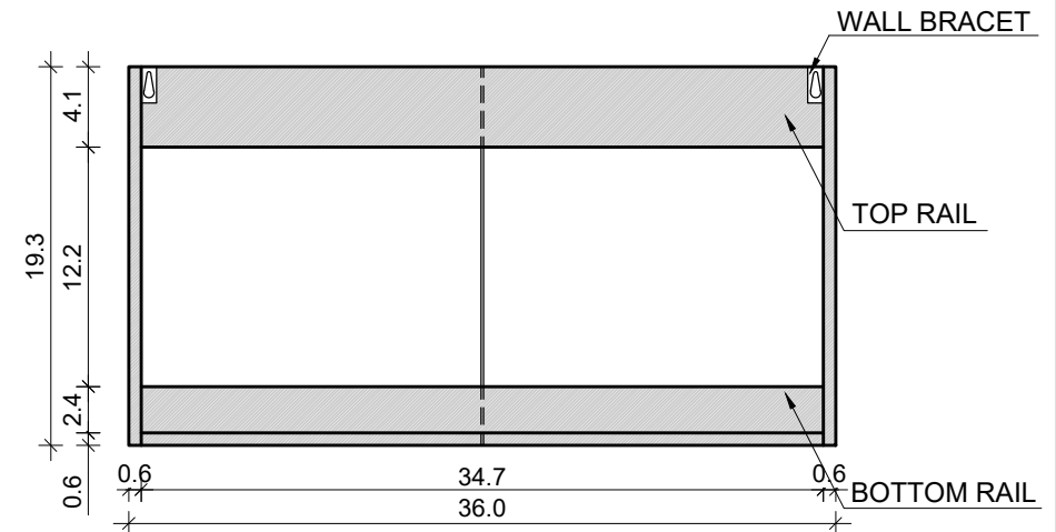
BACK VIEW
