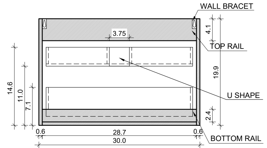
BACK VIEW
