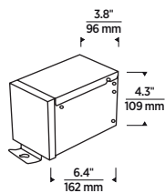
Magnetic Transformer
