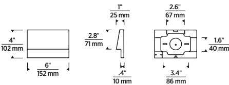
Krysen Outdoor Wall/Step Light
