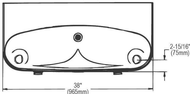
WALL LAYOUT
