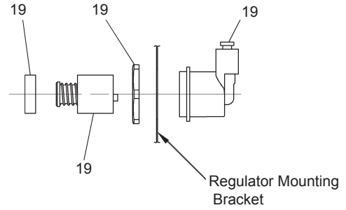
Figure 9 Regulator Assembly
