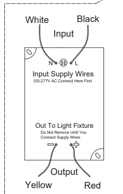
Wiring diagram
