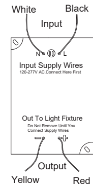
Wiring diagram
