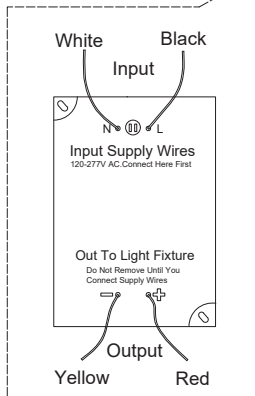
Wiring diagram
