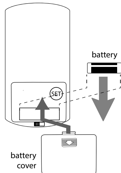
REMOTE CONTROL (back)
