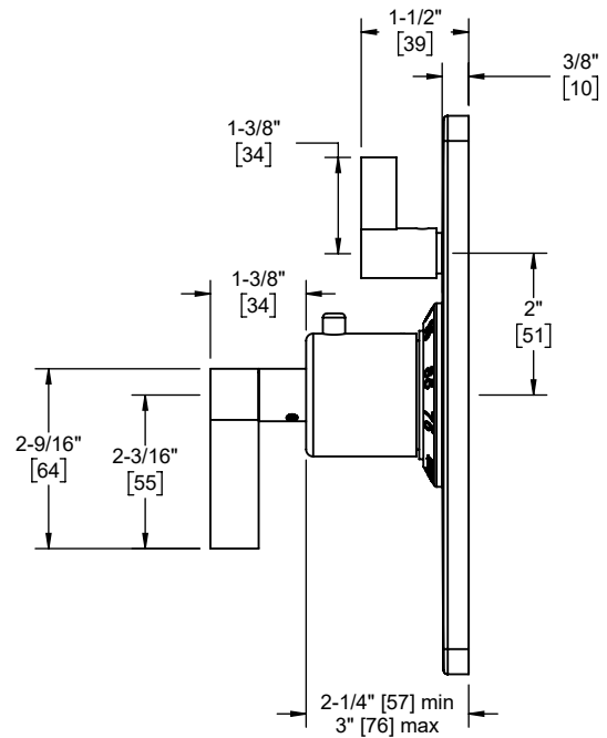
TO-THC1L-40X
