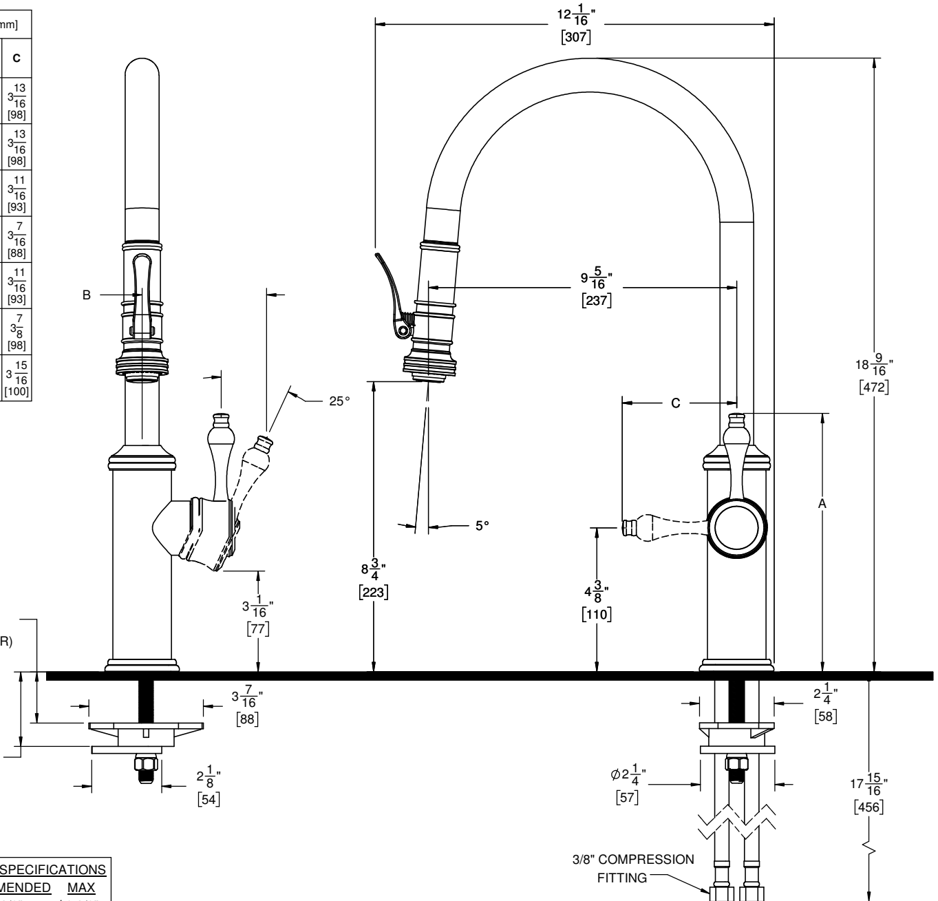
CF-K10-100SQ-42-ZZ SHOWN
