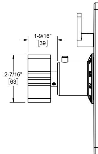
TO-THC1L-37X side view
