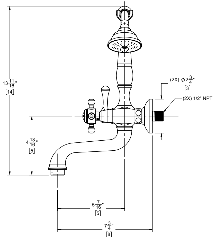
1506-D-47.FR SHOWN
