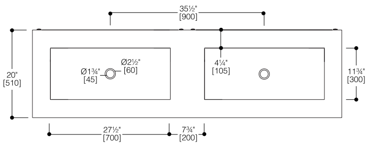
VANITY TOP VIEW
