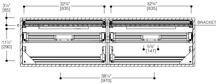
WALL DRILLING SCHEME FOR VANITY
