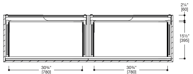
BOTTOM DRAWER VIEW
