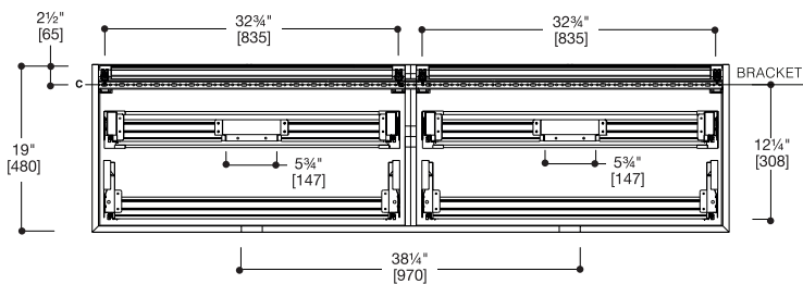
WALL DRILLING SCHEME FOR VANITY
