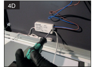
Close the infrared (IR) switch box (C)
