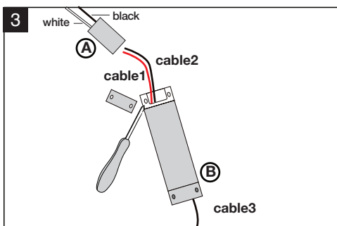
Connect cable (1) red / (2) black from the transformer (B) to the electrical box (A).
