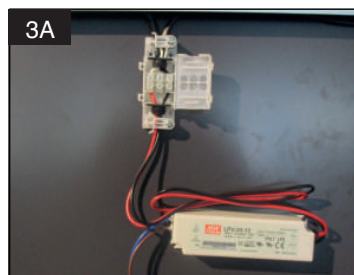
Now the black cable from the transformer (B) is connected with the black cable from the electrical box (A) and the red cable from the transformer (B) is now connected with the white cable from the electrical box (A).
