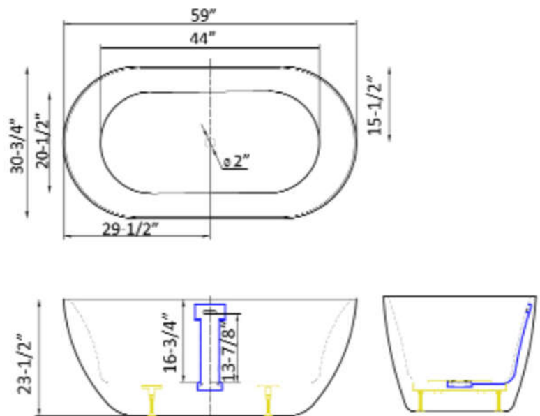
(Air jet configuration if system is added, more info on page 2.)
