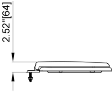
Left view
