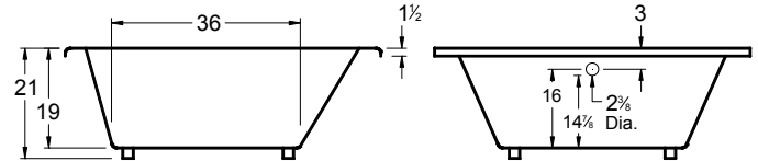
All bathtub dimensions are ± 1/2"
