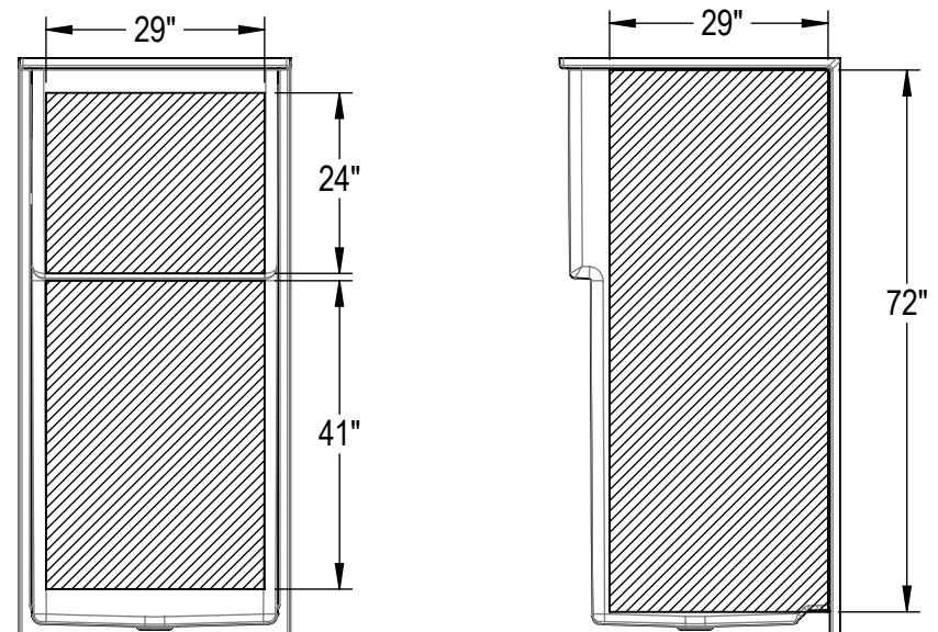
Full Wall Reinforcement Option
