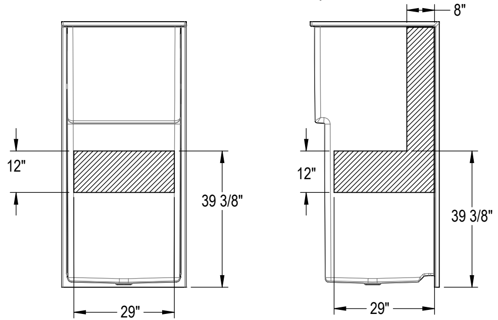
FHA Reinforcement Option
