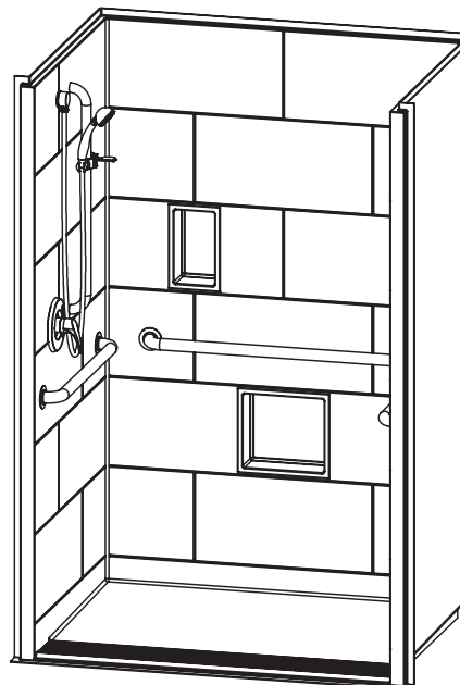
Left wall left fixture placement configuration shown with optional soap dish
