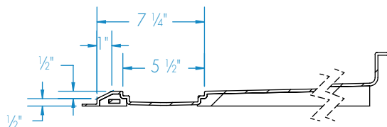
SECTION B-B Integral Pre-levleed Base trench grate (included), not shown
