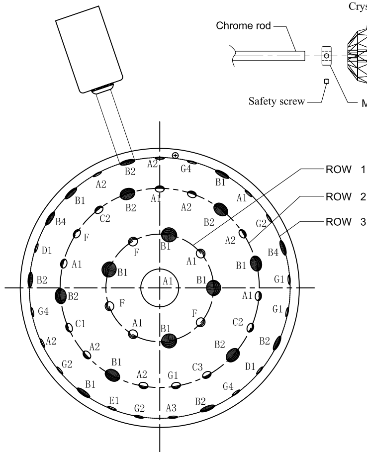
Bottom view
