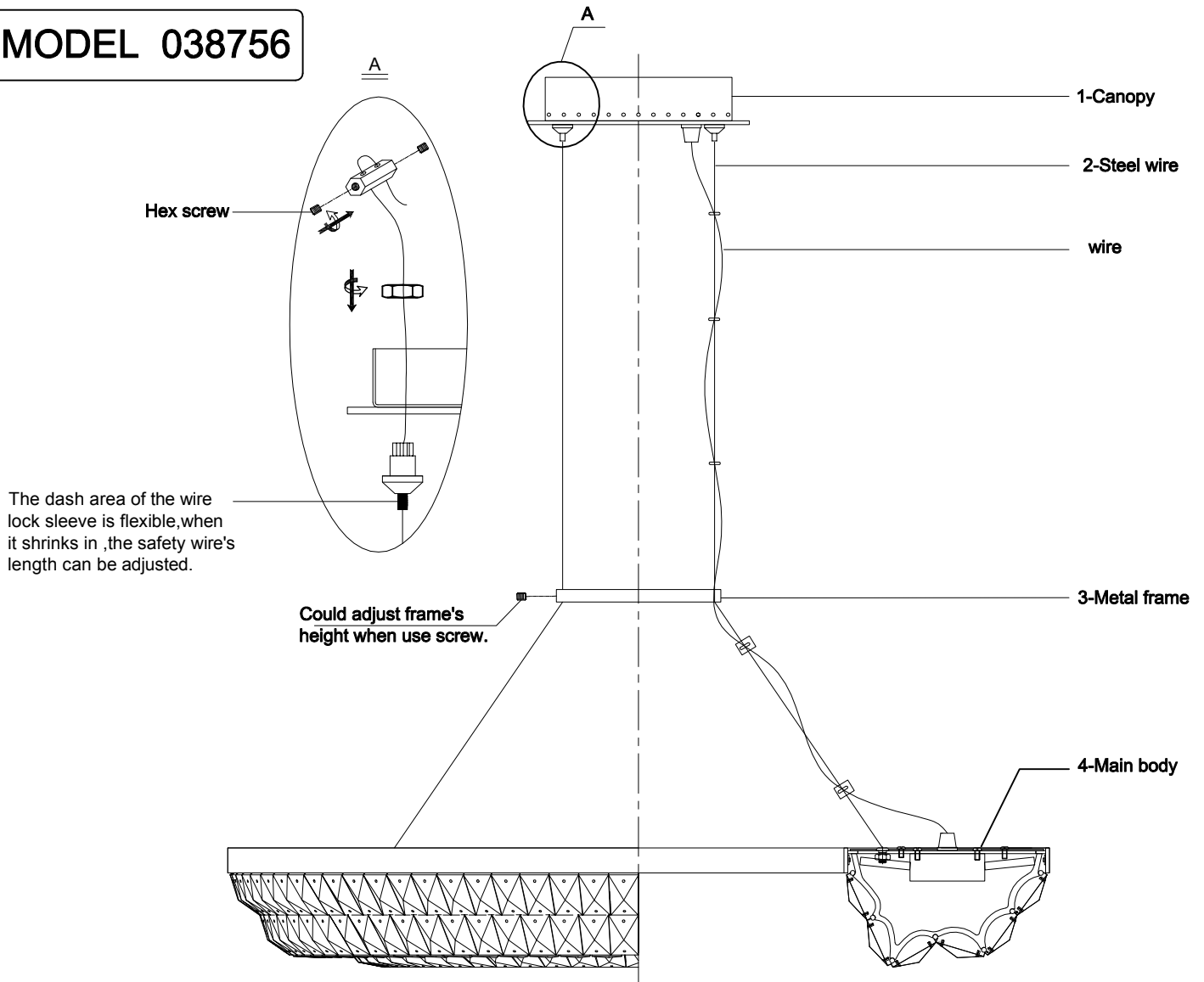
Wire connecting view
