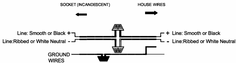
Wiring Diagram
