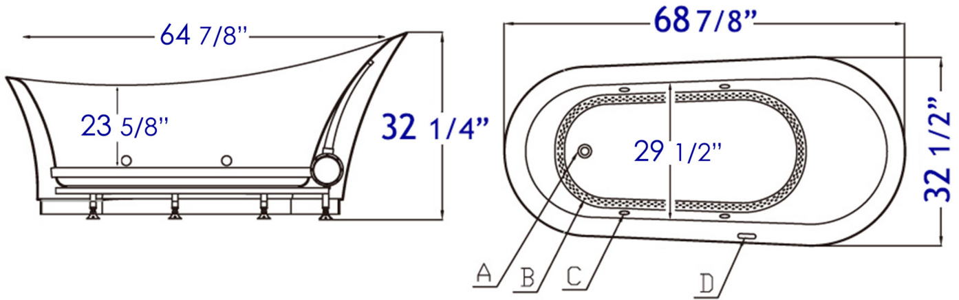
A: Drain B: Air Holes C: LED Lights D: Control Panel
