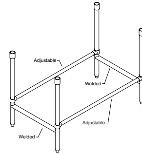
94 Series Includes front & Rear Adjustable Cross Bracing (Shown Above)
