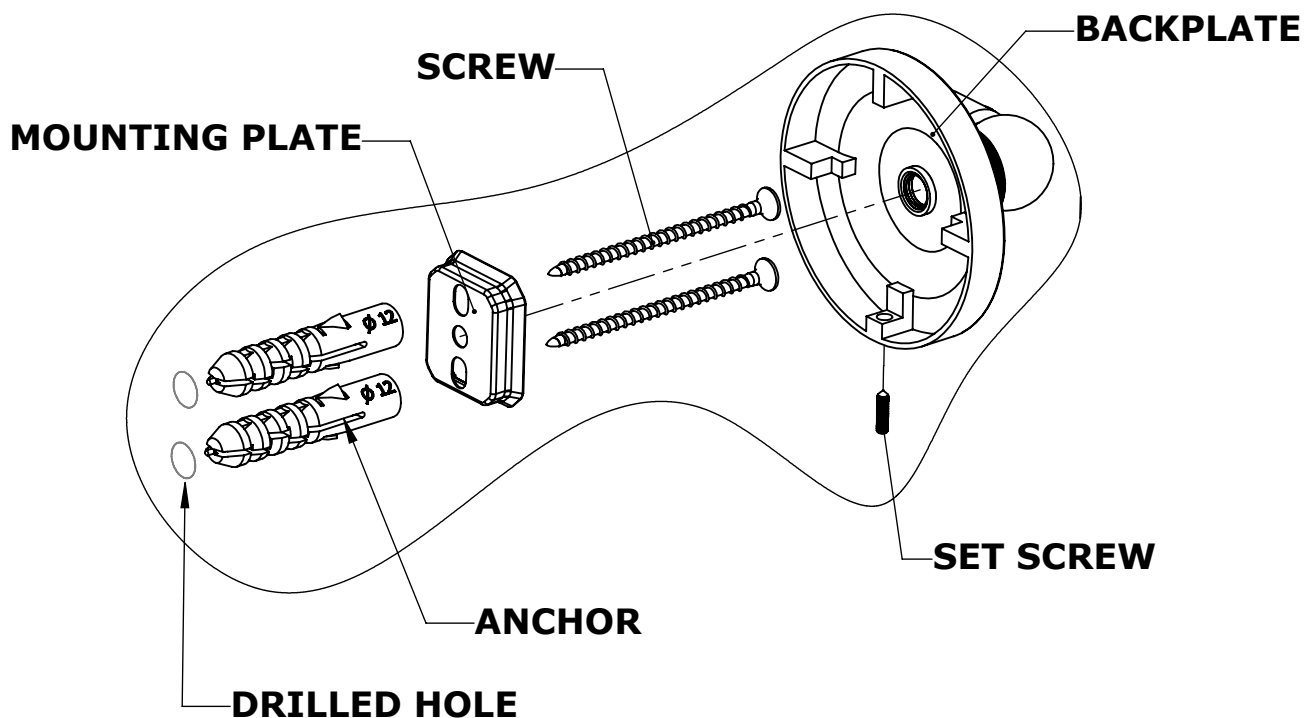
DETAIL O
