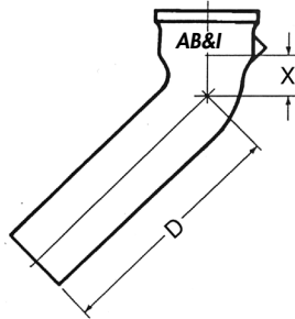
LONG EIGHTH BEND
