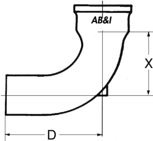
SHORT SWEEP BEND
