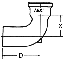
QUARTER BEND, REDUCING
