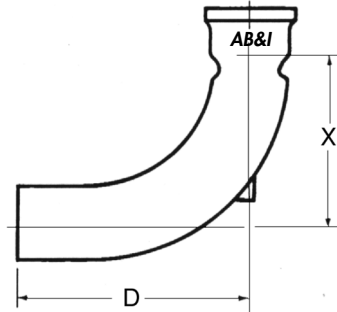
LONG SWEEP BEND, REDUCING
