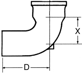
QUARTER BEND
