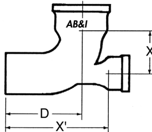
QUARTER BEND w/ Low Heel Inlet
