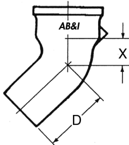
EIGHTH BEND
