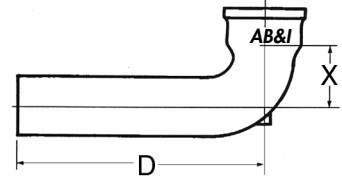
LONG QUARTER BEND
