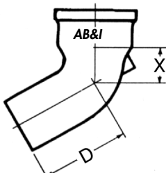
SIXTH BEND
